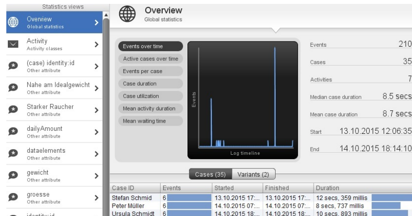
Abbildung 5.8: Disco Statistics
