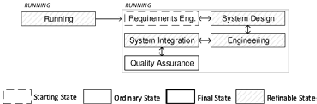
Figure 2.6: Individual State Model for proCollab Process Instance [MR17c]
