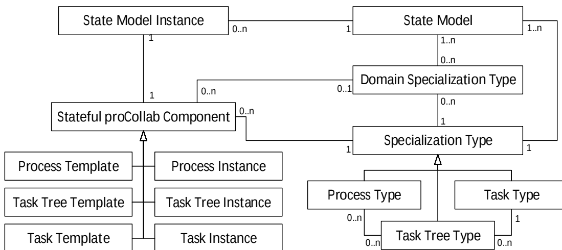
Figure 2.7: Specialization Entities [MR17c]
