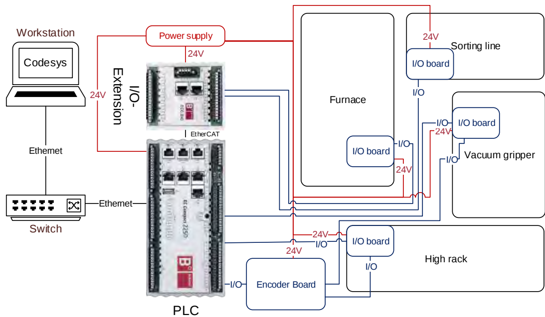
Figure 4.1: Factory Simulation Hardware Components
