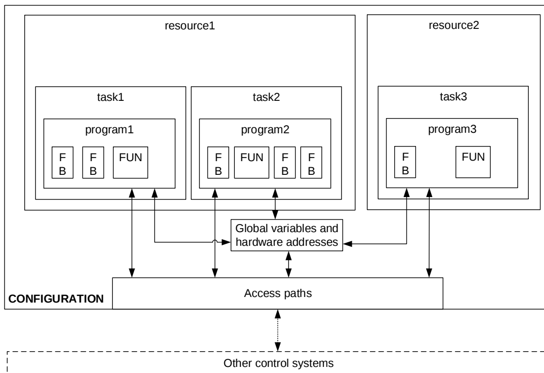
Figure 2.8: IEC 61131-3 Software Model [3]
