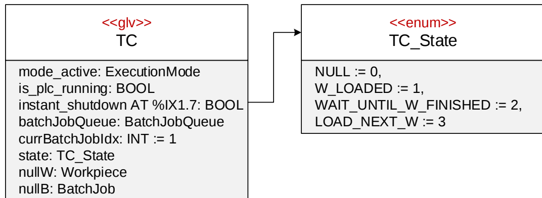
Figure 4.7: Task Configurator – Global Variable List and State
