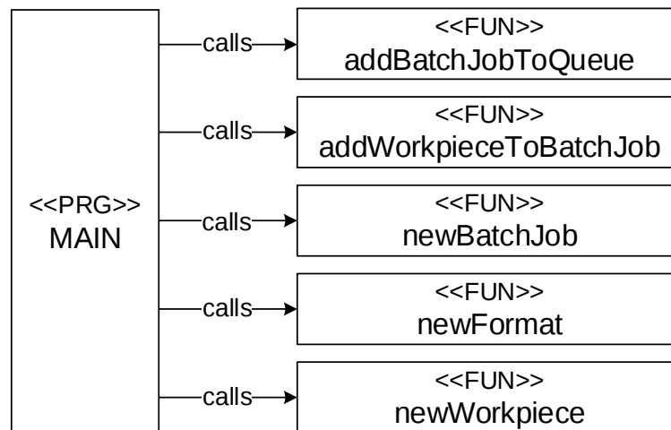
Figure 3.5: FUNs, used by MAIN
