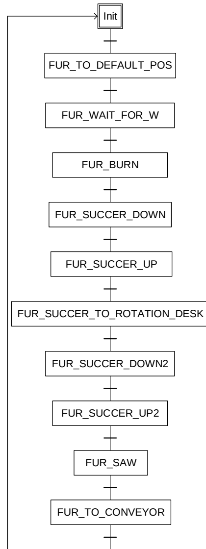
Figure 4.15: FUR Single Mode – SFC Process Sequence
