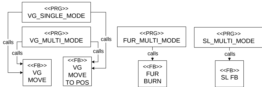
Figure 3.4: POUs with Call Relations to VG, FUR and SL
