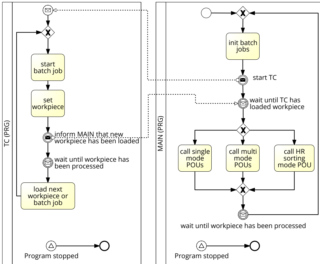
Figure 3.6: TC and MAIN – Process Model
