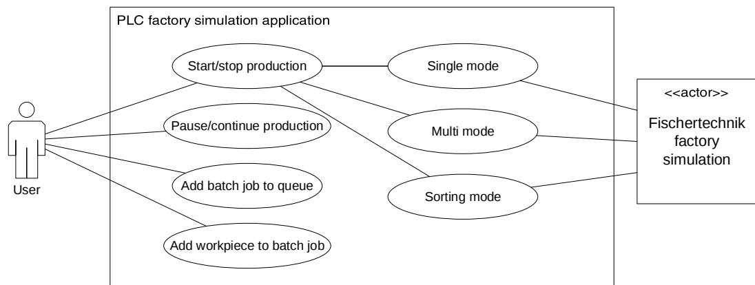
Figure 3.1: Factory Simulation – Use Case Diagram
