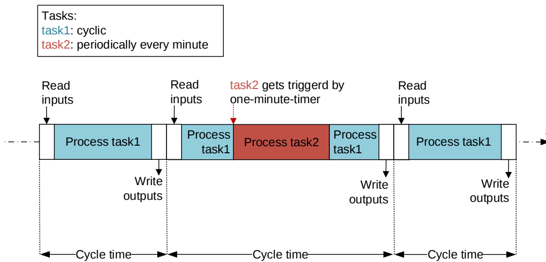
Figure 2.5: PLC Task Displacement
