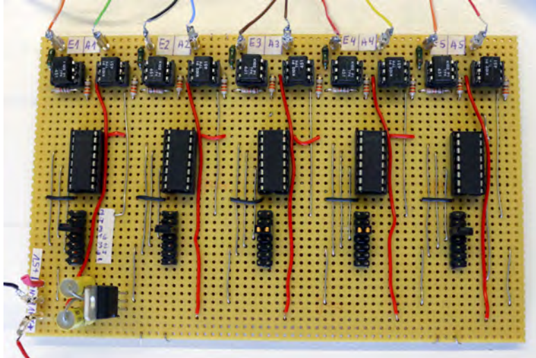
Figure 2.7: Encoder Board – Components
