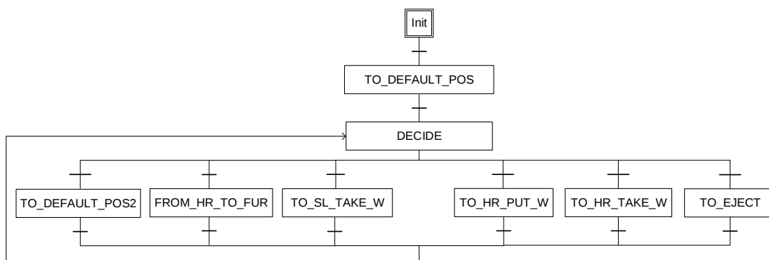
Figure 4.13: VG Multi Mode – SFC Process Sequence
