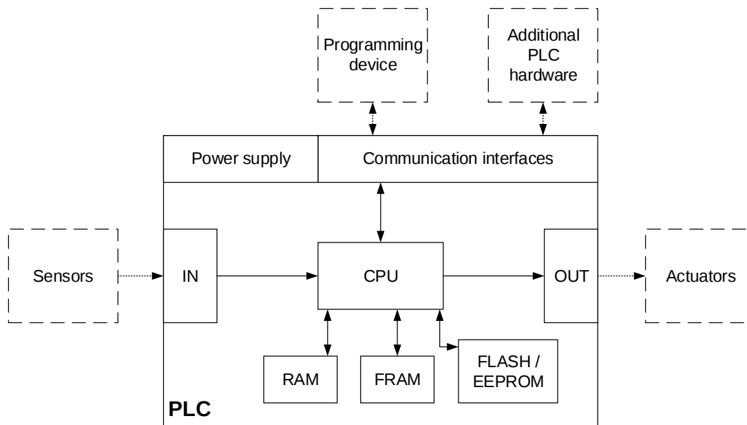
Figure 2.3: PLC Hardware Structure [4]
