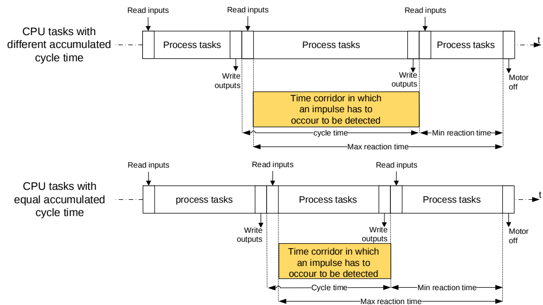
Figure 2.6: PLC Task Execution
