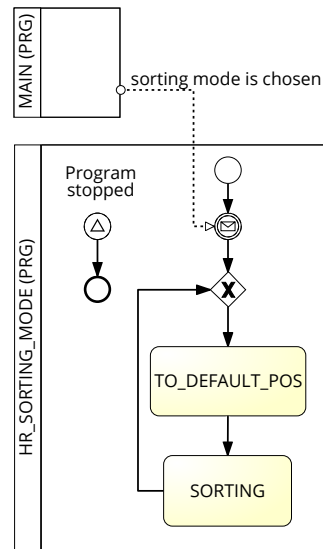
Figure 3.9: Sorting Mode – Process Model
