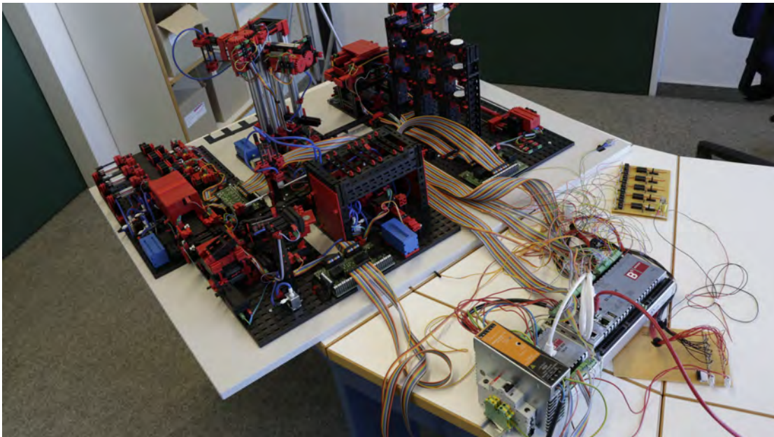
Figure 4.2: Fischertechnik Factory Simulation with PLC and Wiring
