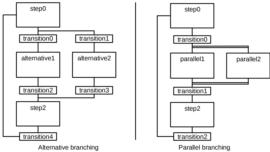
Figure 2.12: SFC Networks – Alternative and Parallel Branching
