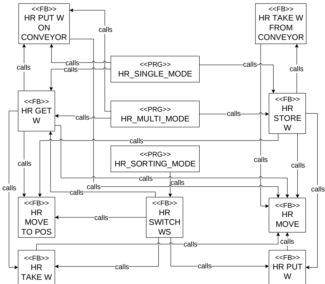
Figure 3.3: HR POUs and their Call Relations
