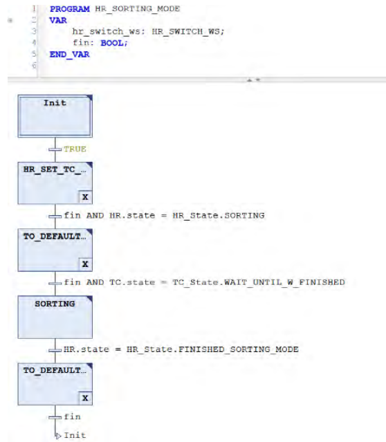
Figure A.1: HR_SORTING_MODE – SFC Steps
