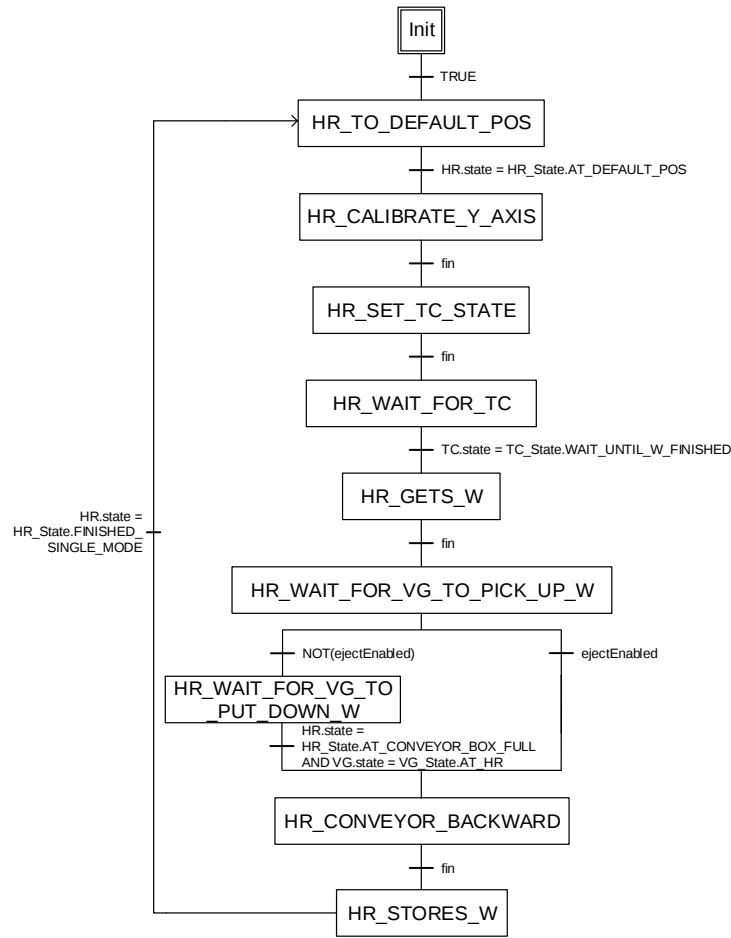
Figure 4.10: HR_SINGLE_MODE SFC Process Sequence
