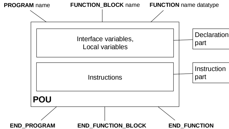
Figure 2.9: Program Organization Unit – Structure [9]
