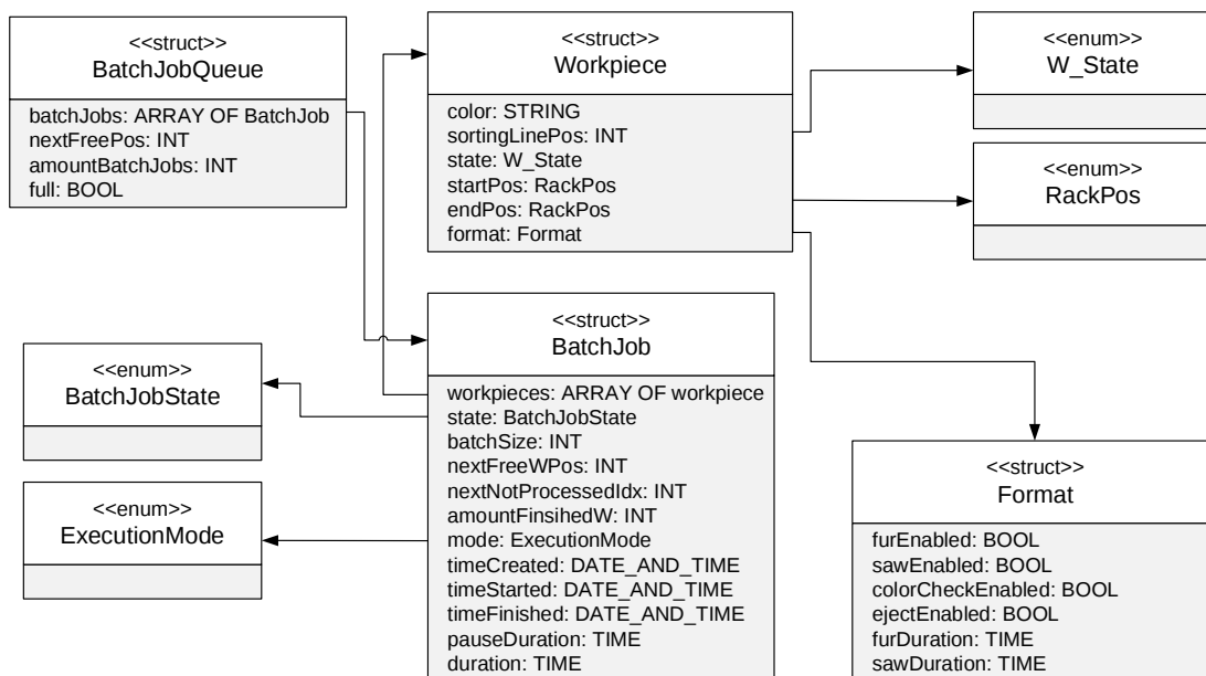
Figure 3.10: Data Structures – Class Model
