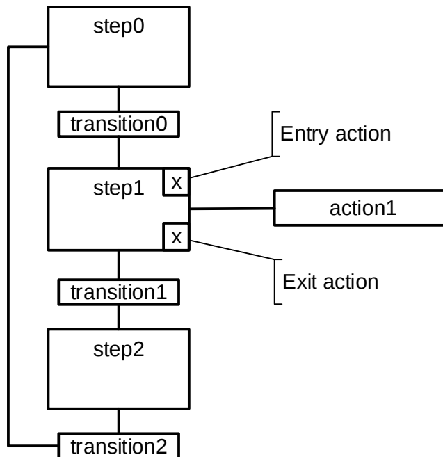
Figure 2.11: SFC Network Elements and their Composition
