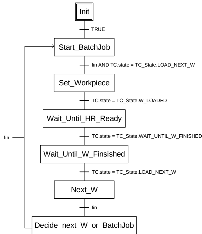
Figure 4.8: TC_POU Process Sequence
