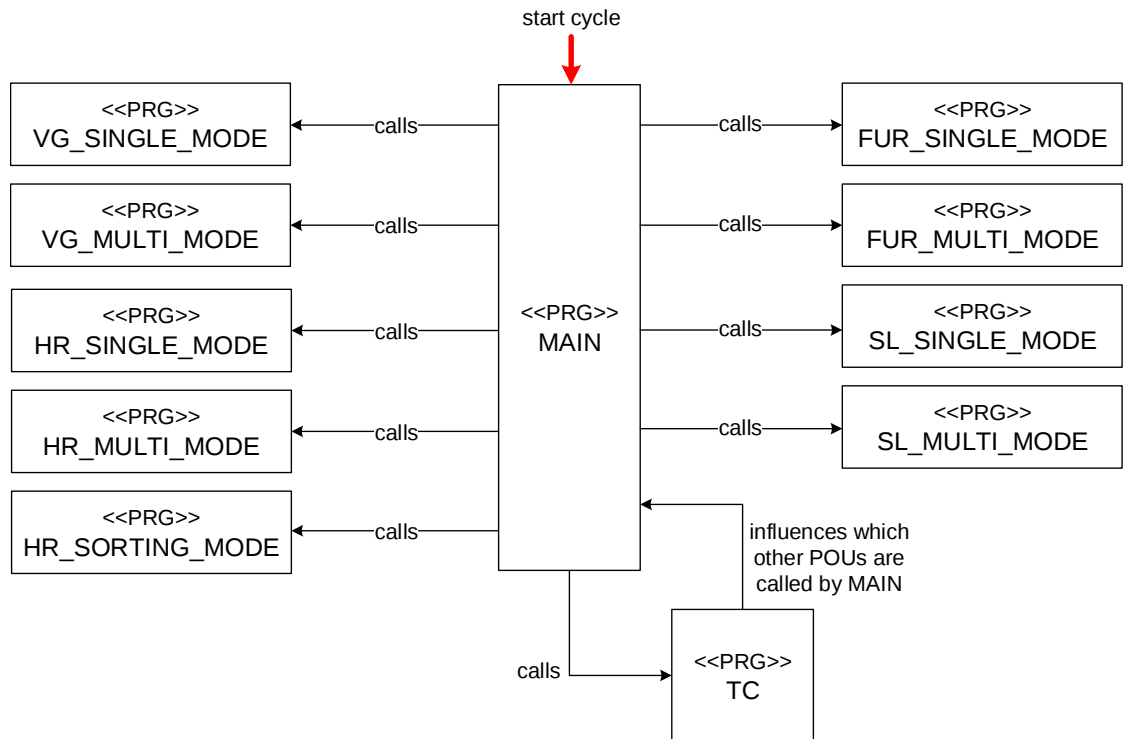
Figure 3.2: Factory Simulation – PRGs Overview
