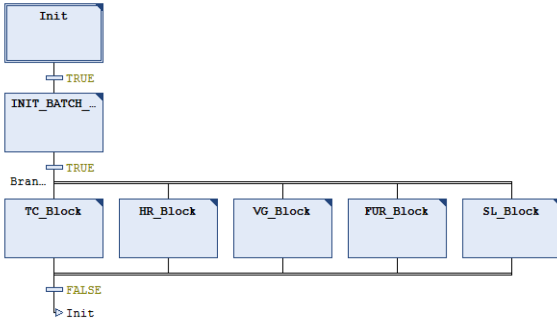
Figure 4.6: MAIN PRG – Graphical Implementation
