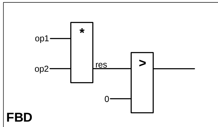
Figure 2.10: FBD Code Example
