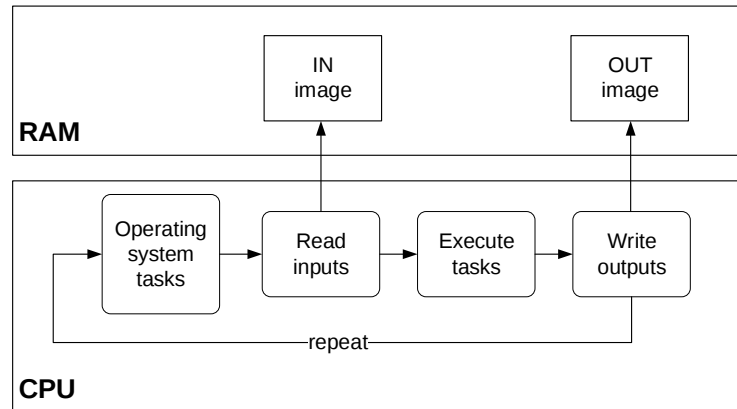
Figure 2.4: PLC Code Execution Cycle (based on [3])
