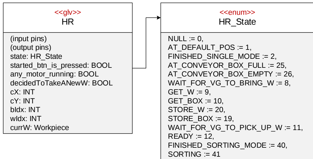
Figure 4.9: HR GLV and HR_State Enum
