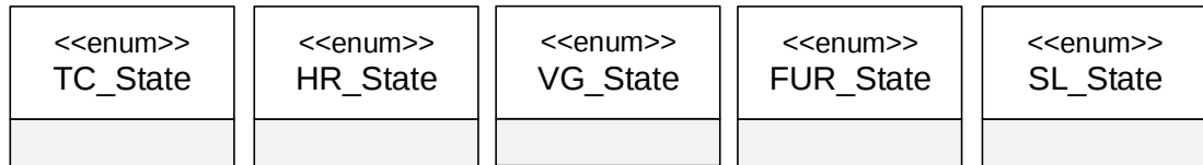
Figure 3.11: Enums – Overview
