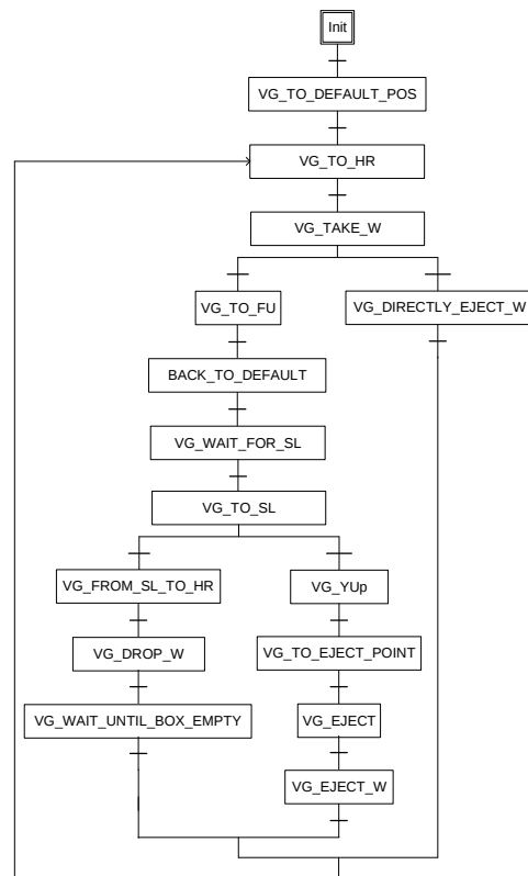
Figure 4.12: VG Single Mode – SFC Process Sequence
