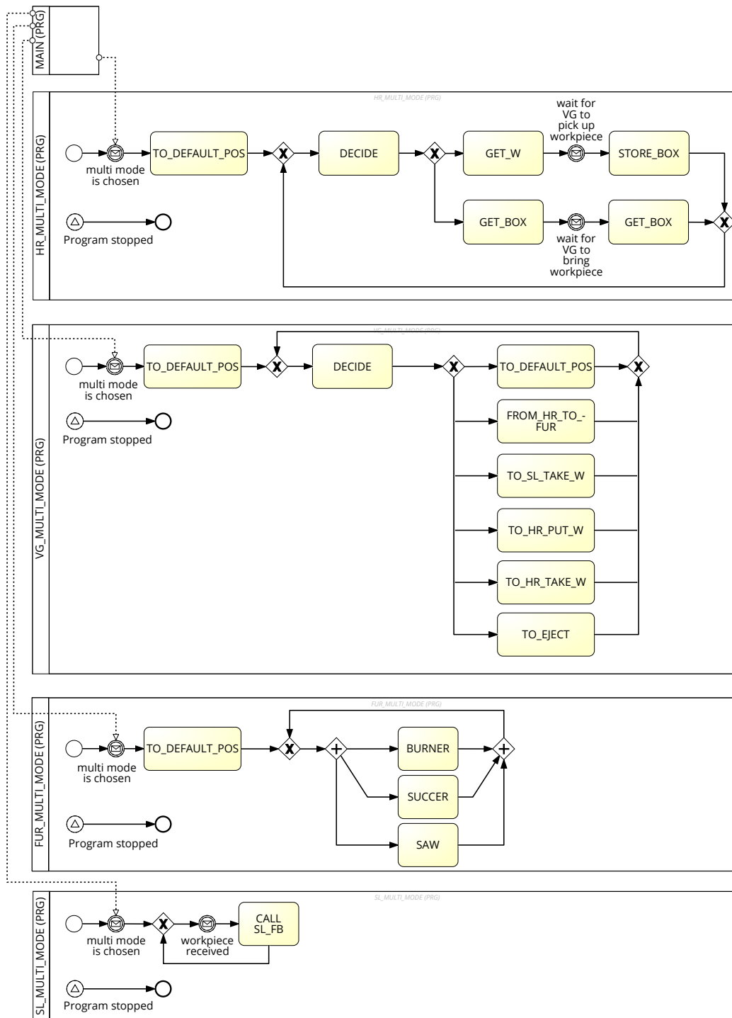
Figure 3.8: Multi Mode – Process Model
