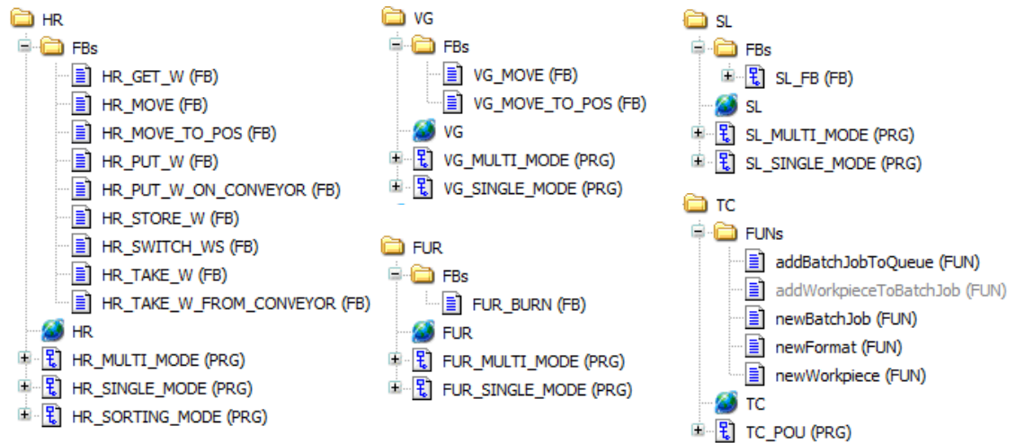
Figure 4.5: Factory Stations and Task Configurator – File Structure
