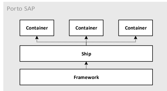
Figure 5.1: Overview about the different layers in the PORTO SAP 1 .
