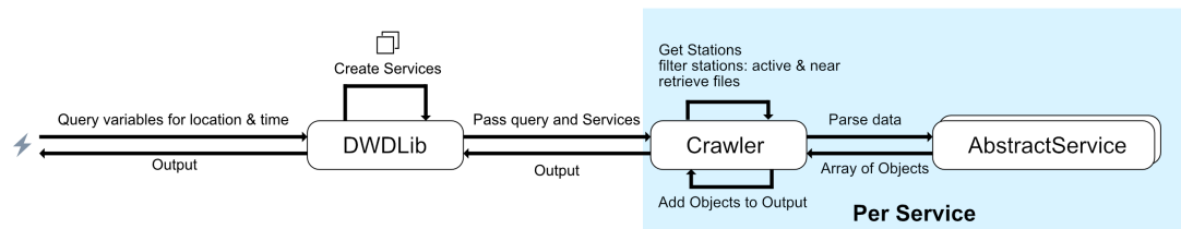
Figure 5.13: A short introduction to the inner workings of the library including core components.
