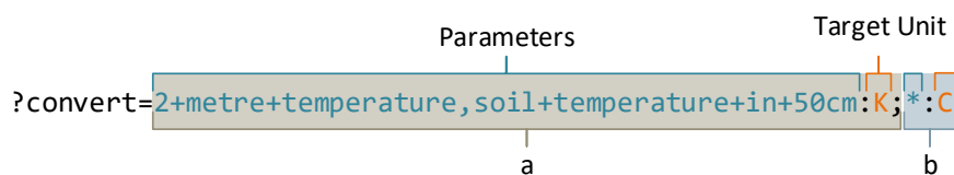
Figure 5.8: Explanation of a sample conversion string that contains two separate conversions, one using specific parameters and one that uses the wild card notation.
