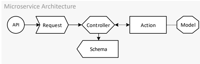
Figure 5.11: Adapted life-cycle similar to a minimalistic Porto implementation.
