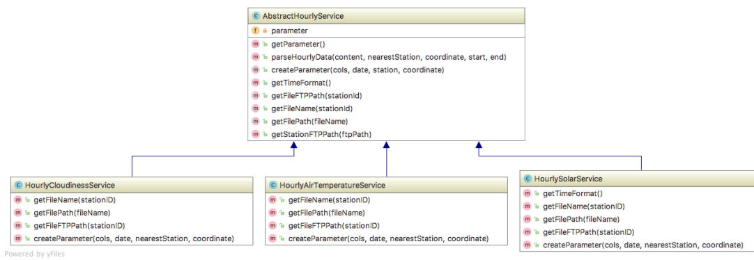
Figure 5.14: Class hierarchy of the service classes, with a selection of three out of eight subclasses.
