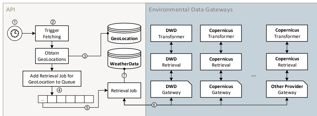
Figure 5.6: Shows the complete cycle between a time triggered fetching of GeoLocations up to the retrieval and storage of data inside one common WeatherData table.
