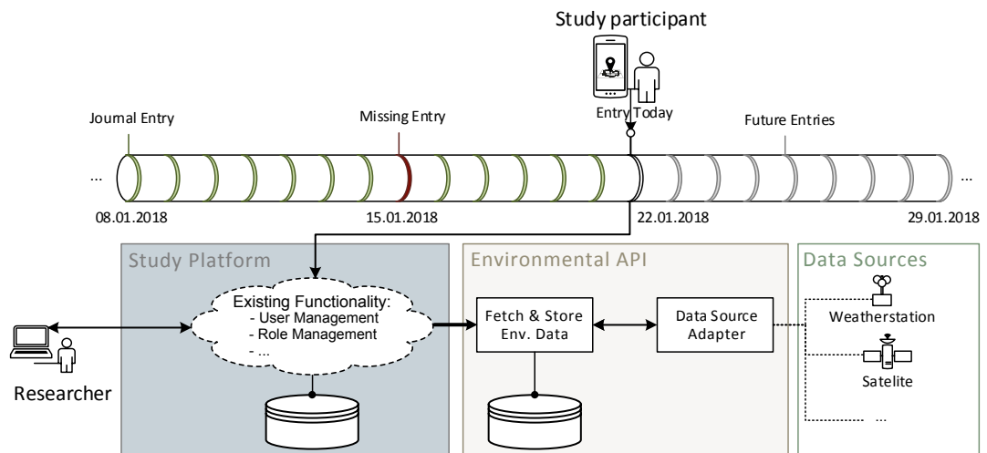
Figure 3.1: Proposed procedure for the participants of the study by visualizing the (daily) journal entries that consist of a geolocation and a date on a timeline. Those entries, in turn, allow the API to provide environmental data to the user.
