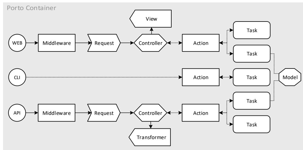
Figure 5.2: Interactions between the Components in Porto SAP 2 .
