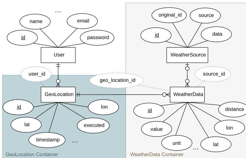
Figure 5.5: ER Diagram of all models introduced by the two implemented containers.
