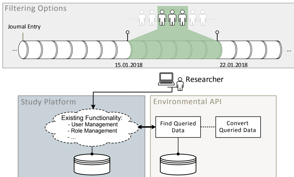
Figure 3.2: Proposed procedure for a researcher that includes querying the environmental database to retrieve data for one or more participants and optionally converting from one unit (e.g., °C) to another one (e.g., °K).
