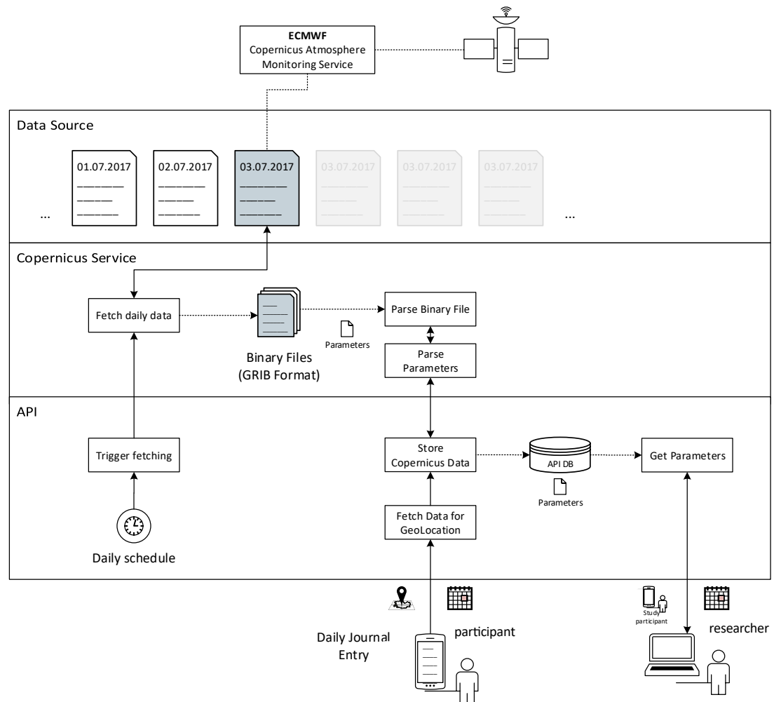
Figure 5.9: Planned Copernicus Wrapper including planned API access.
