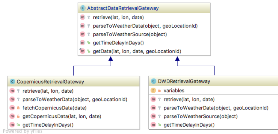
Figure 5.4: Class Diagram showing the abstract parental class and the two subclasses for DWD and Copernicus data.
