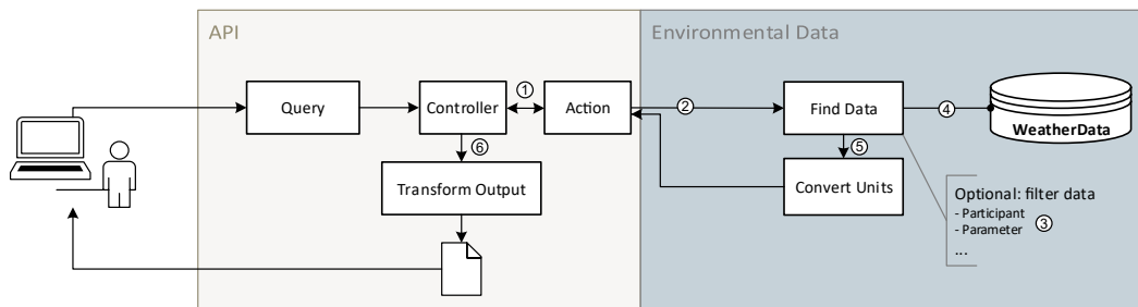
Figure 5.7: Researcher querying the API for environmental data via the provided endpoints.
