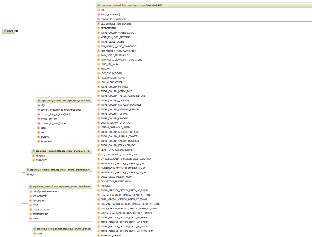
Figure B.1: All available enums inside of the wrapper including available methods and fields.
