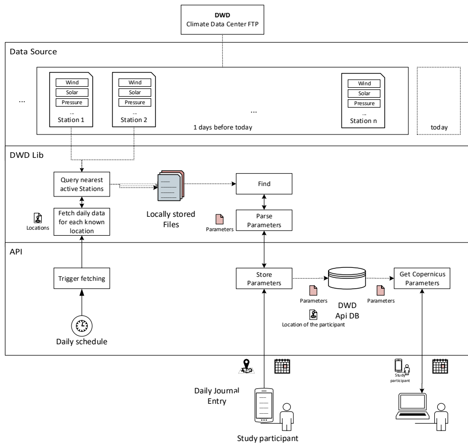
Figure 5.12: Planned integration of the library onto the RESTful environmental API.
