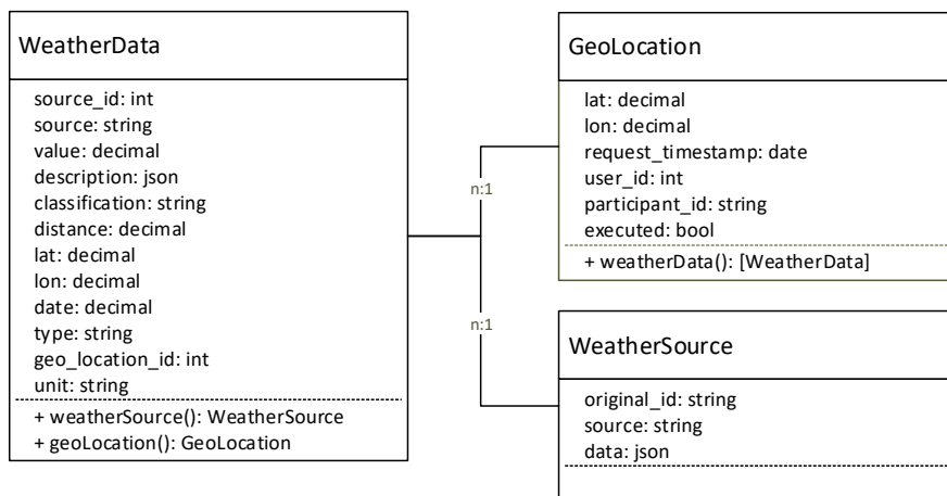
Figure 5.3: Class Diagram that shows how GeoLocations , WeatherData and WeatherSource are connected. All public functions provide a means to retrieve linked models.
