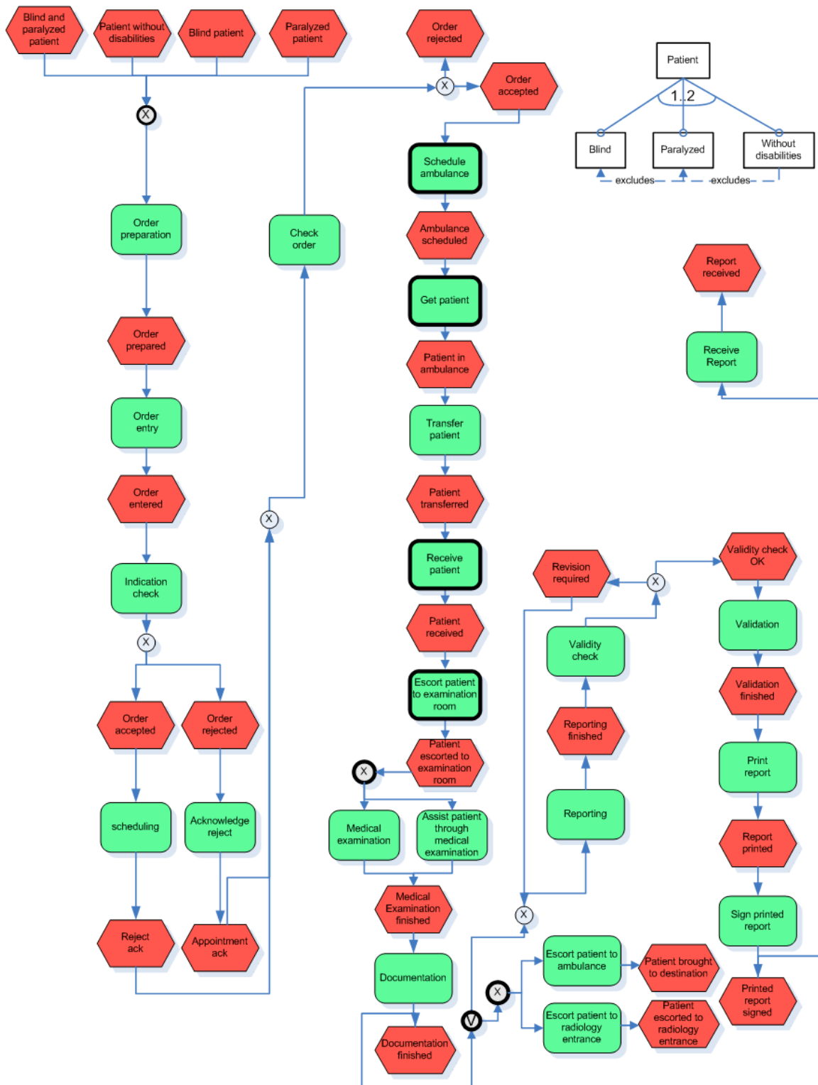
Figure 56: Modeling the healthcare running example using Feature-EPC
