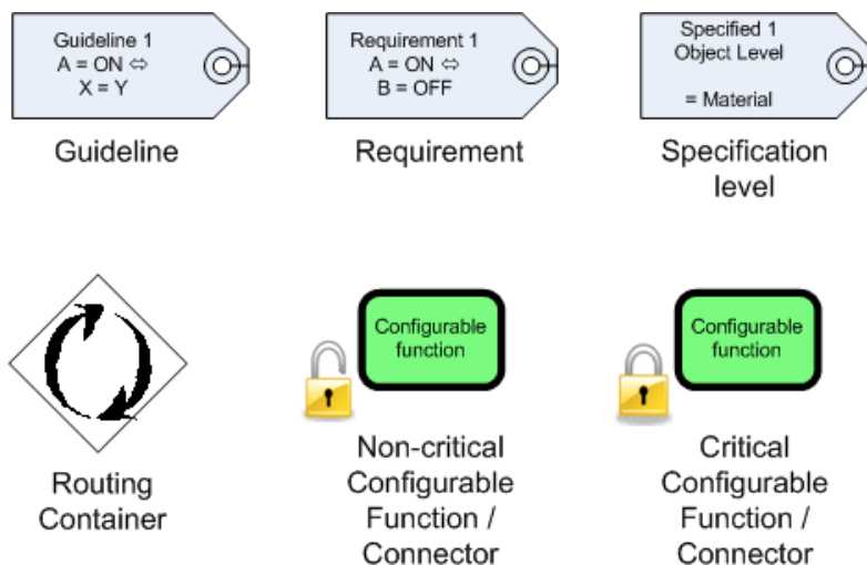
Figure 5: Configurable attributes [5]
