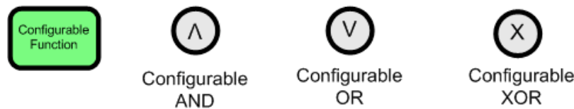
Figure 4: Configurable nodes [5]
